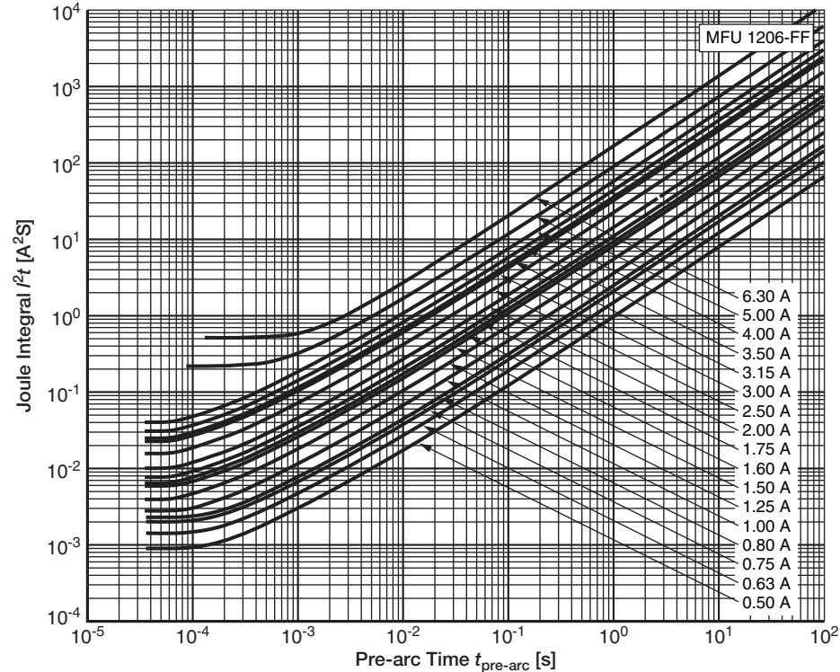
Typical I^2t vs. t_{\text{pre-arc}} characteristic of MFU 1206 (1)
