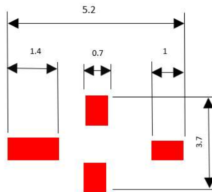
PCB Footprint
