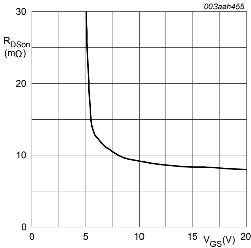
Fig. 7. Drain-source on-state resistance as a function of gate-source voltage; typical values T_j = 25\text{ °C}; I_D = 15\text{ A}
