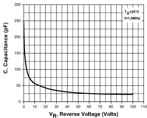
Capacitance for CMSH3-100MA
