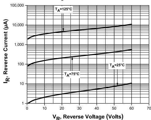
Leakage Current for CMSH3-60MA
