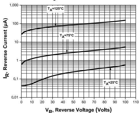
Leakage Current for CMSH3-100MA
