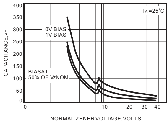
Fig.6 TYPICAL CAPACITANCE
