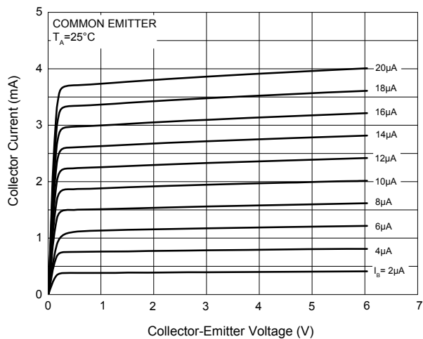
Fig. 1 - Static Characteristics
