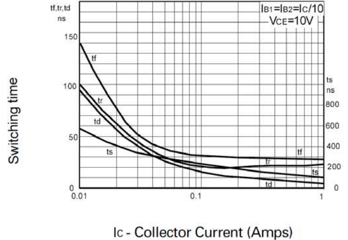
Switching Speeds
