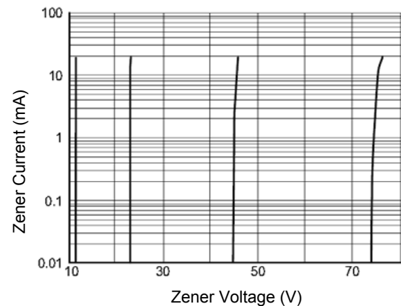
Figure 6. Zener Breakdown Characteristics
