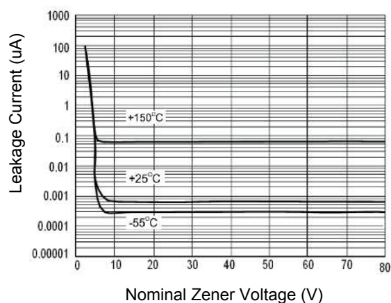
Figure 7. Typical Leakage Current
