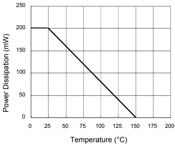
Figure 3. Power Dissipation vs. Ambient Temperature
