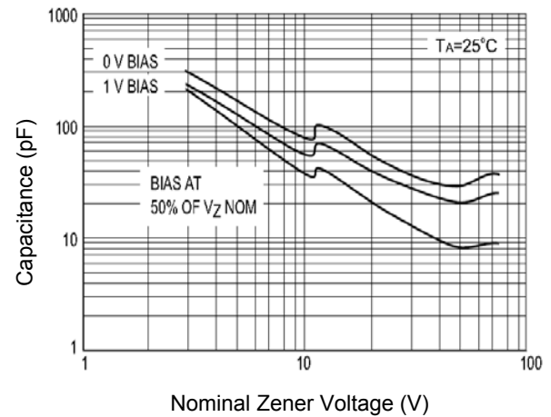
Figure 4. Typical Capacitance
