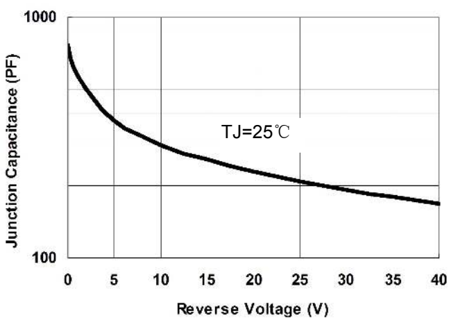
Fig.1-Typical Junction Capacitance
