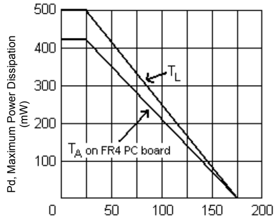
T_L – Lead Temperature (°C) 3/8" from body or T_A on FR4 PC Board
