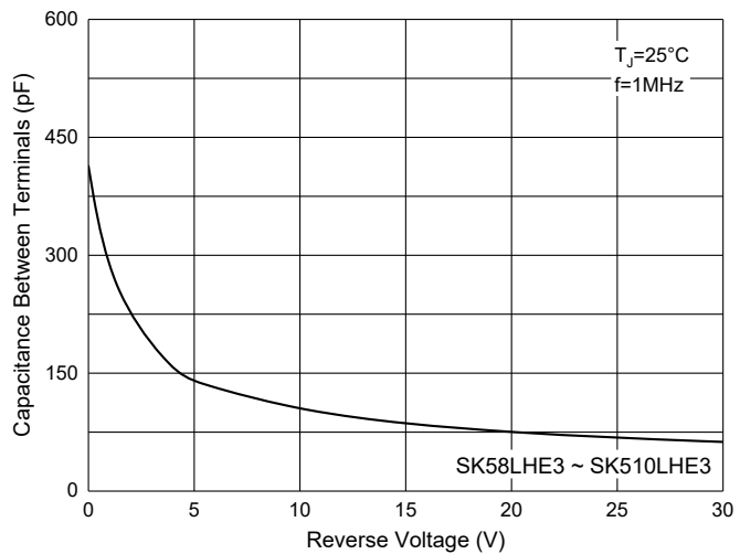
Fig. 11 - Capacitance Characteristics
