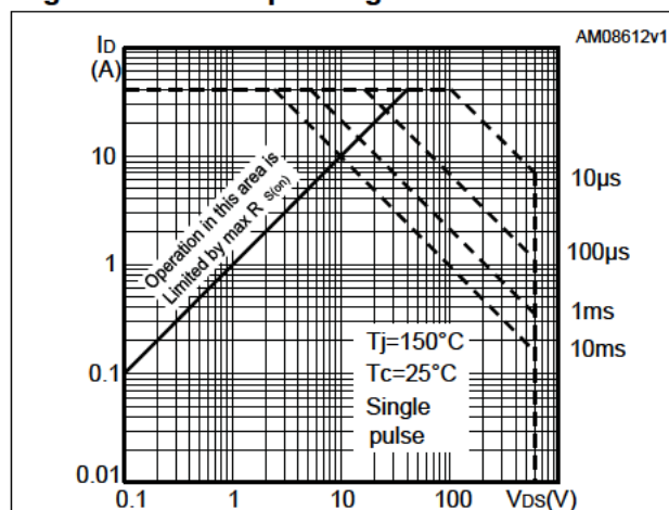
Figure 6. Safe operating area for DPAK, IPA
