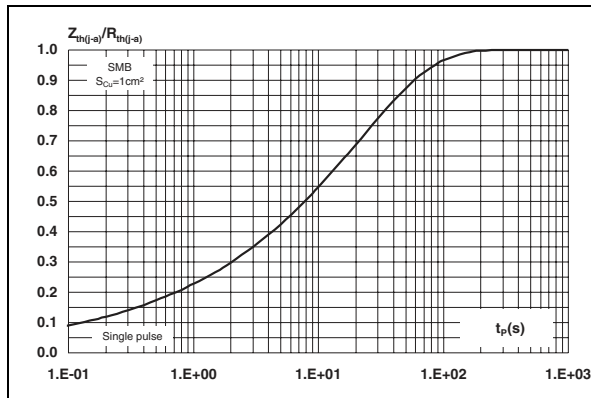
Figure 5. Relative variation of thermal impedance junction to ambient versus pulse duration, SMB (epoxy FR4, copper thickness = 35 \mu m)
