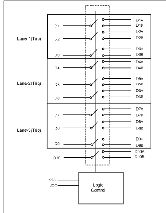
C-PHY
