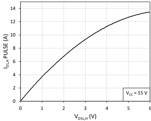
Fig. 5. Pulsed Drain current ( I_{DSL,H} PULSE) vs. drain-to-source voltage ( V_{DSL,H} ) at T = 25^\circ\text{C}
