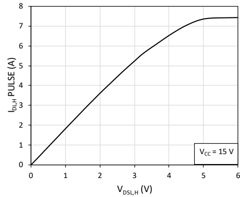
Fig. 6. Pulsed Drain current ( I_{DSL,H} PULSE) vs. drain-to-source voltage ( V_{DSL,H} ) at T = 125^\circ\text{C}
