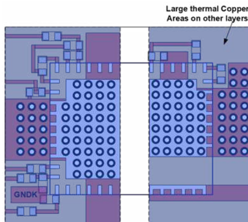
Step 3. Place large copper areas on other layers. Make all thermal copper areas as large as possible! Keep high and low side layouts separate on all PCB layers.
