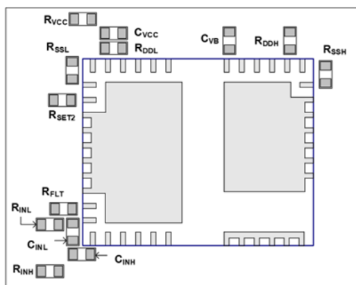
IC Component placement
