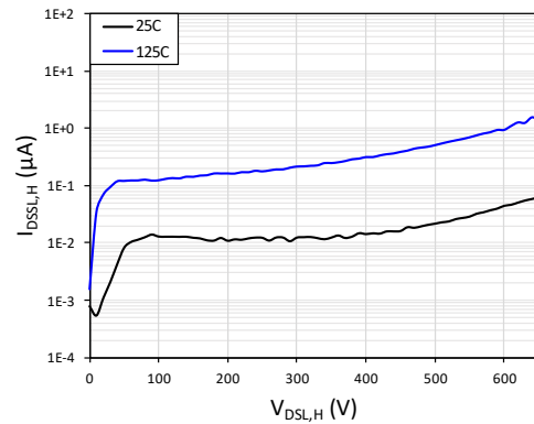
Fig. 8. Drain-to-source leakage current ( I_{DSSL,H} ) vs. drain-to-source voltage ( V_{DSL,H} )
