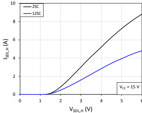
Fig. 7. Source-to-drain reverse conduction voltage ( I_{SDL,H} )
