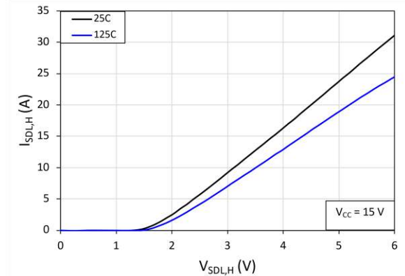
Fig. 7. Source-to-drain reverse conduction voltage ( I_{SDL,H} )
