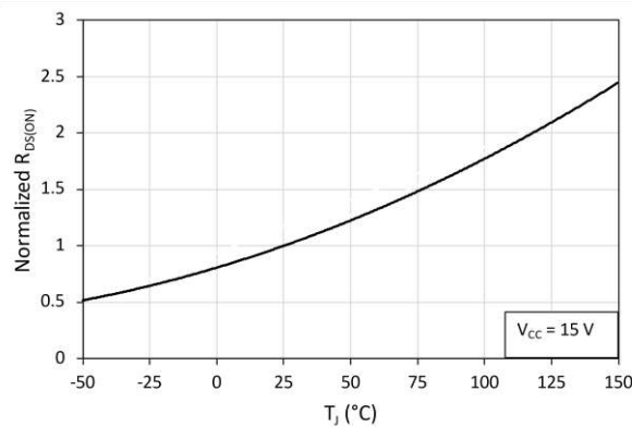
Fig. 10. Normalized on-resistance ( R_{DSL,H(ON)} ) vs. junction temperature ( T_J )
