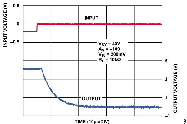
Figure 47. Positive Overload Recovery, V_{SY} = \pm 5 V
