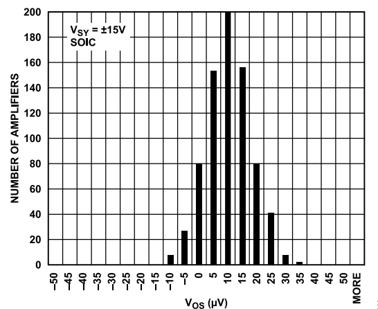
Figure 14. Offset Voltage ( V_{OS} ) Distribution, V_{SY} = \pm 15\text{ V}
