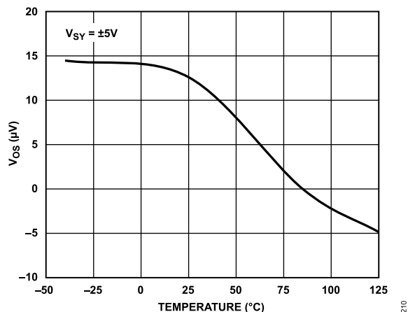
Figure 12. Offset Voltage ( V_{OS} ) vs. Temperature, V_{SY} = \pm 5\text{ V}
