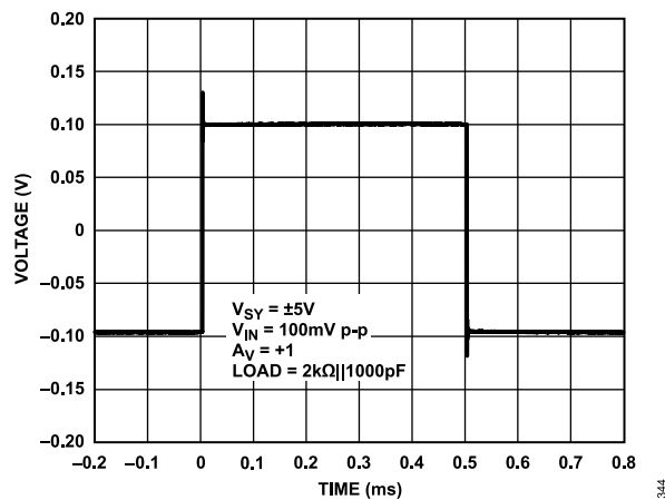
Figure 46. Small Signal Transient Response, V_{SY} = \pm 5 V
