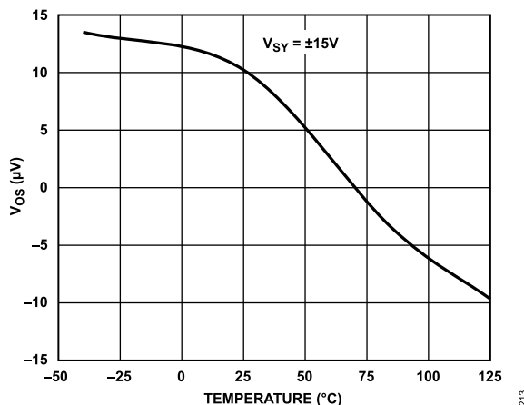
Figure 15. Offset Voltage ( V_{OS} ) vs. Temperature, V_{SY} = \pm 15\text{ V}
