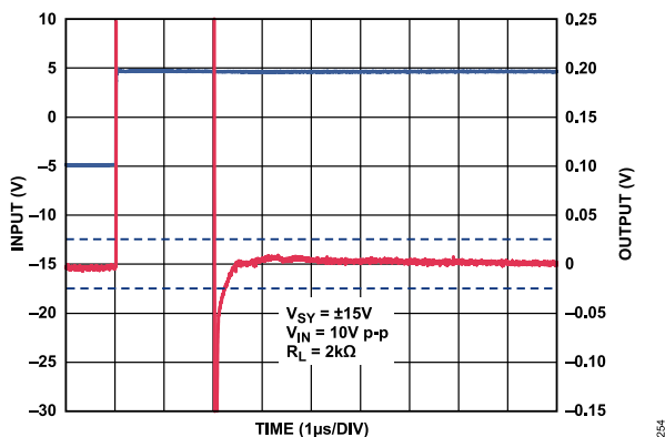
Figure 56. Positive 0.1% Settling Time, V_{SY} = \pm 15\text{ V}
