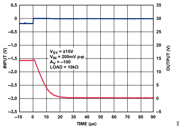
Figure 50. Positive Overload Recovery, V_{SY} = \pm 15 V
