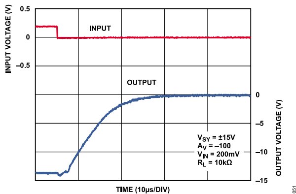
Figure 51. Negative Overload Recovery, V_{SY} = \pm 15 V
