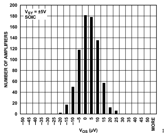
Figure 11. Offset Voltage ( V_{OS} ) Distribution, V_{SY} = \pm 5\text{ V}
