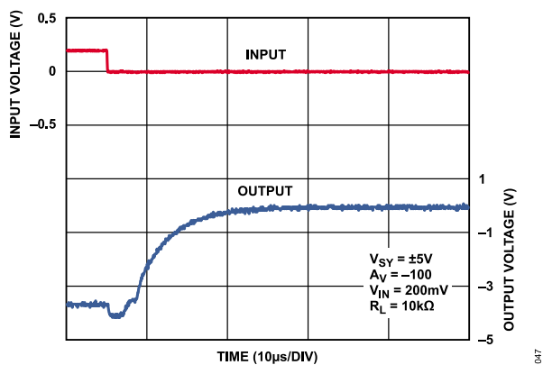
Figure 48. Negative Overload Recovery, V_{SY} = \pm 5 V
