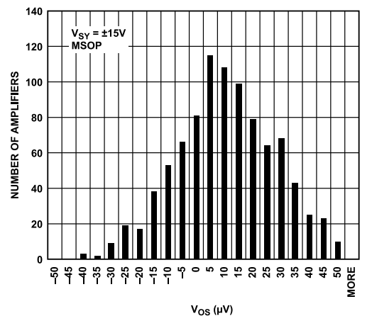
Figure 13. ADA4077-2 Offset Voltage ( V_{OS} ) Distribution, V_{SY} = \pm 15\text{ V}
