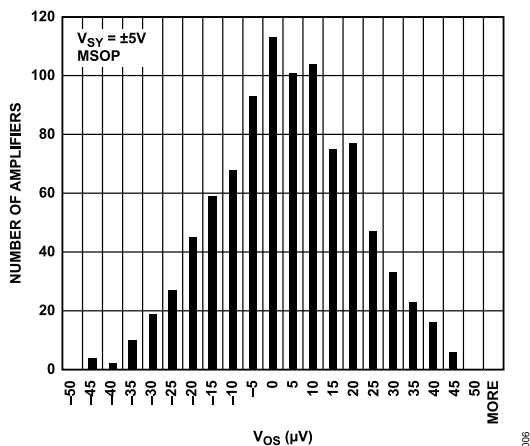
Figure 10. ADA4077-2 Offset Voltage ( V_{OS} ) Distribution, V_{SY} = \pm 5\text{ V}
