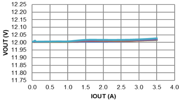
Figure 6. Load Regulation
