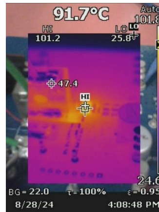
Figure 9. Case Temperature, V_{IN} = 100\text{V} , V_{OUT} = 12\text{V} , I_{OUT} = 3.5\text{A}
