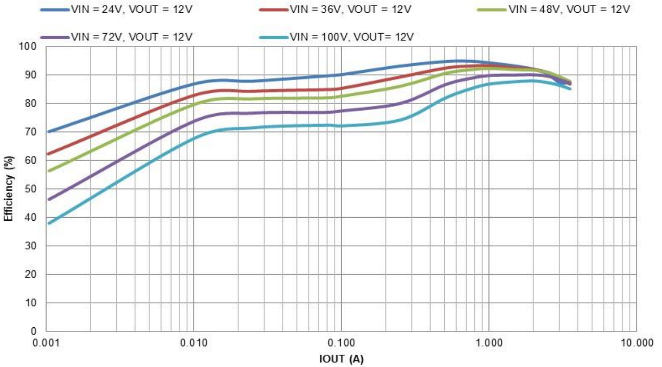
Figure 2. Efficiency vs. Output Current, VOUT = 12V, fsw = 300kHz, L = 68µH
