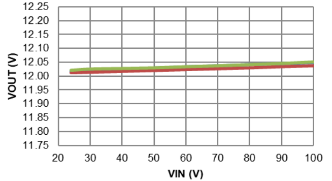
Figure 7. Line Regulation
