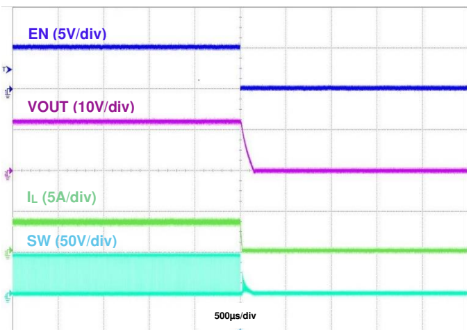
Figure 21. Shutdown using EN, I_{OUT} = 3.5\text{A}
