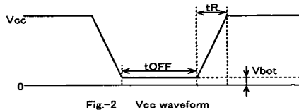
Fig-2 Vcc waveform
