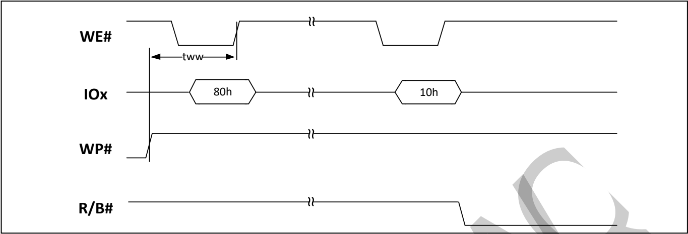
Figure 24 Program Enable
