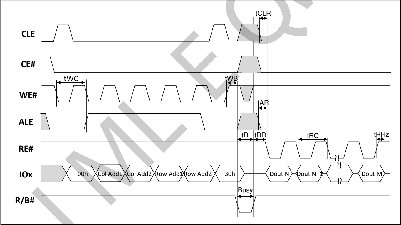
Figure 40 Page Read
