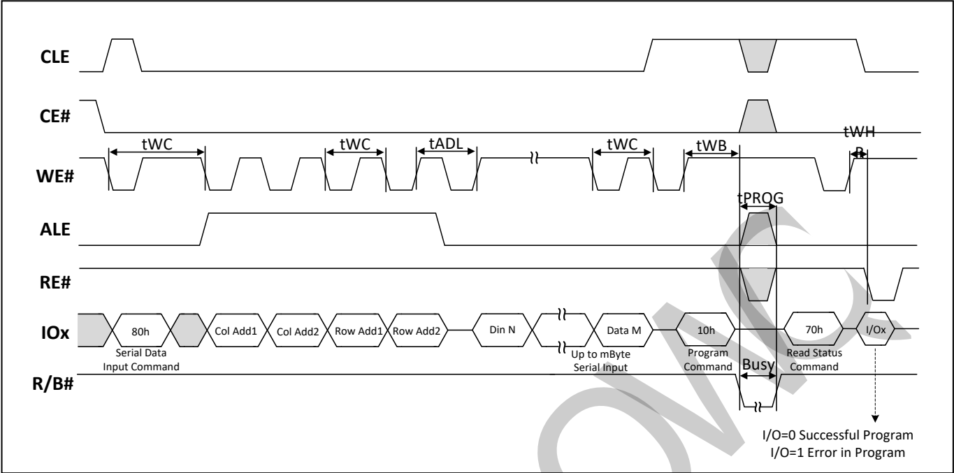
Figure 43 Page Program
