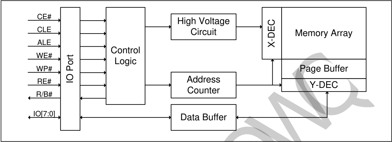
Figure 4 Block Diagram
