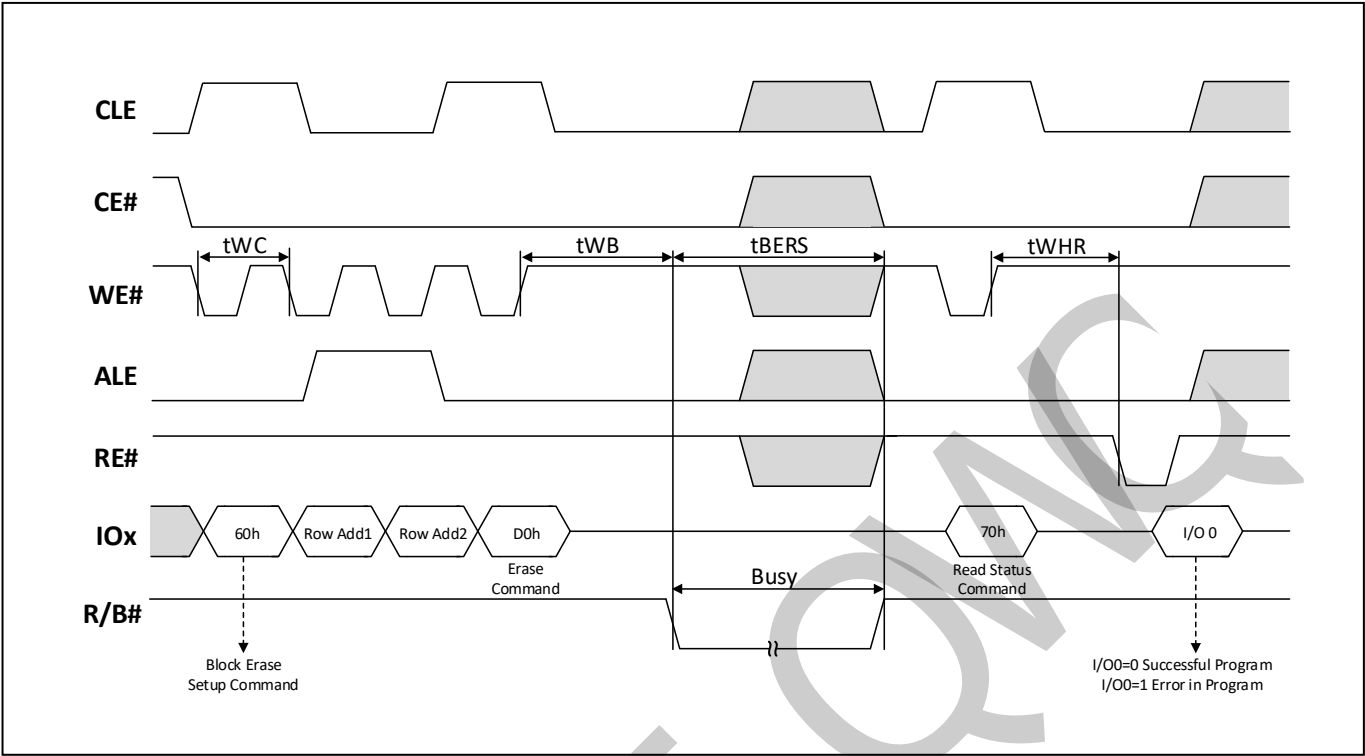
Figure 47 Block Erase
