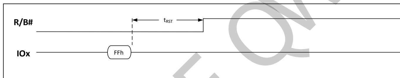
Figure 6 Reset Sequence
