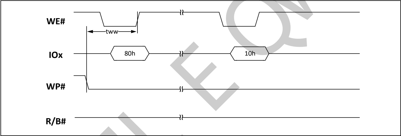
Figure 25 Program Disable
