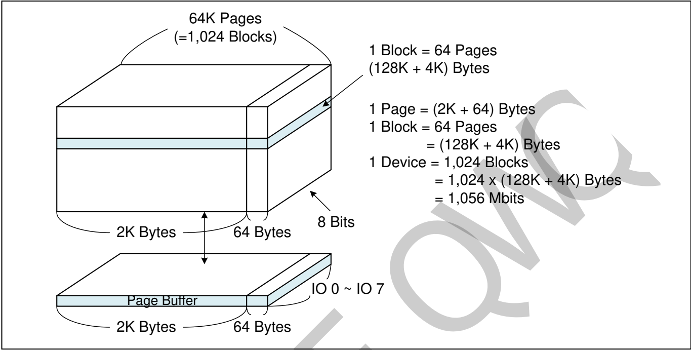
Figure 5 Array Organization
