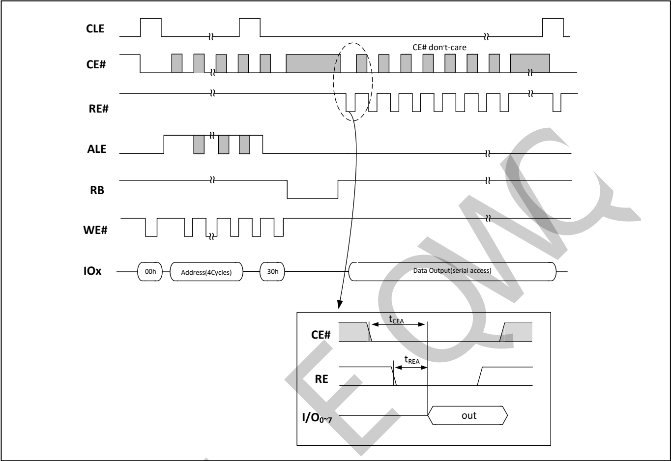
Figure 32 Read Operation with CE# don't-care
