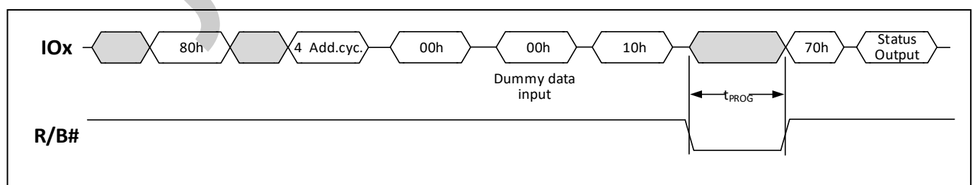
Figure 21 OTP Lock Operation Sequence
