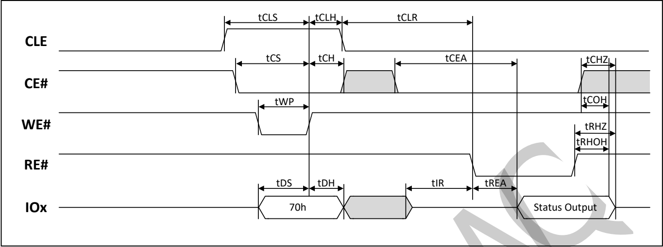
Figure 39 Read Status
