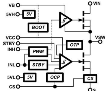
Simplified schematic
