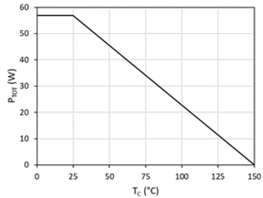
Fig. 20. Power dissipation (P TOT ) vs. case temperature (T C )
