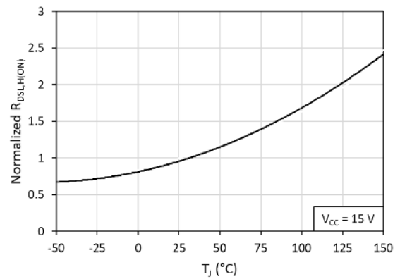
Fig. 10. Normalized on-resistance ( R_{DSL,H(\text{ON})} ) vs. junction temperature ( T_J )
