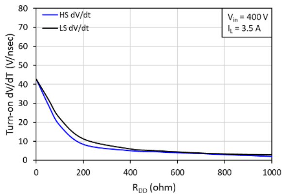
Fig. 19. Slew rate ( dV/dt ) vs. gate drive turn-on current set resistance ( R_{DDL} ) at T = 25^\circ\text{C}
