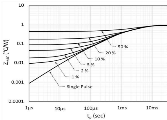
Fig. 21. Max. thermal transient impedance ( Z_{thJC} ) vs. pulse width ( t_p )
