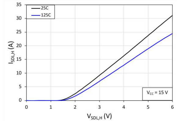
Fig. 7. Source-to-drain reverse conduction voltage ( I_{S,DL,H} ) vs. drain-to-source voltage ( V_{D,SL,H} ) at T = 25\text{ }^{\circ}\text{C} and 125\text{ }^{\circ}\text{C}
