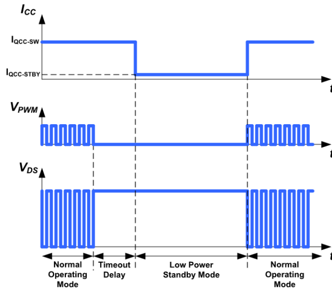
Fig. 26. Autonomous Low Power Standby Mode timing diagram
