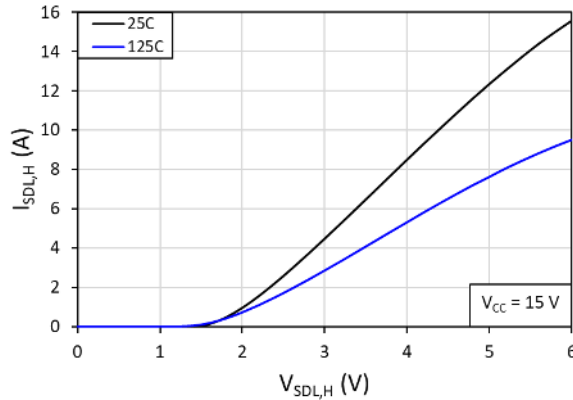
Fig. 7. Source-to-drain reverse conduction voltage ( I_{SDL,H} ) vs. drain-to-source voltage ( V_{DSL,H} ) at T = 25^\circ\text{C} and T = 125^\circ\text{C}
