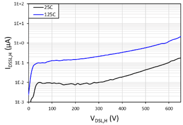
Fig. 8. Drain-to-source leakage current ( I_{DSSL,H} ) vs. drain-to-source voltage ( V_{DSL,H} ) at T = 25^\circ\text{C} and T = 125^\circ\text{C}
