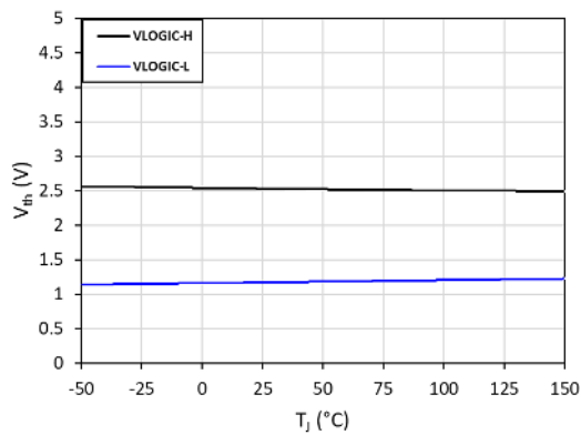
Fig. 9. V_{th} and V_{th} vs. junction temperature ( T_J )
