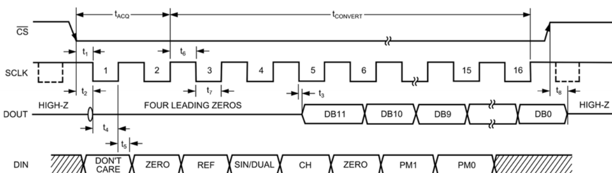
Figure 14: TSA7887's Detailed Serial Interface Timing Diagram.
