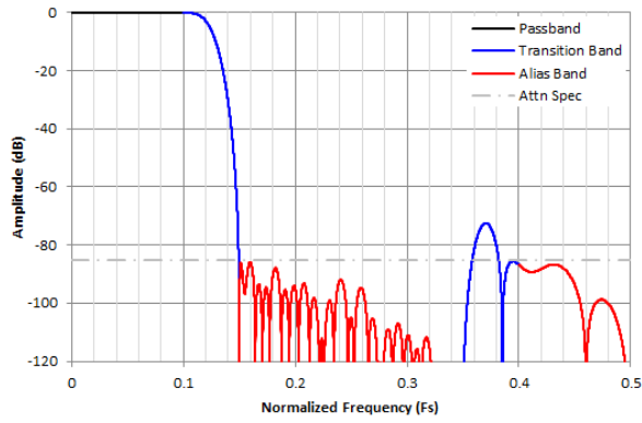
Figure 8-25. Complex Decimation by 4 Filter Response
