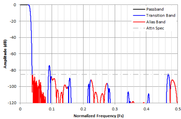
Figure 8-29. Complex Decimation by 16 Filter Response
