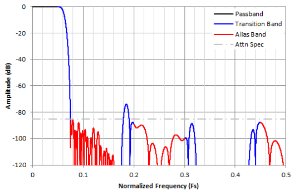
Figure 8-27. Complex Decimation by 8 Filter Response
