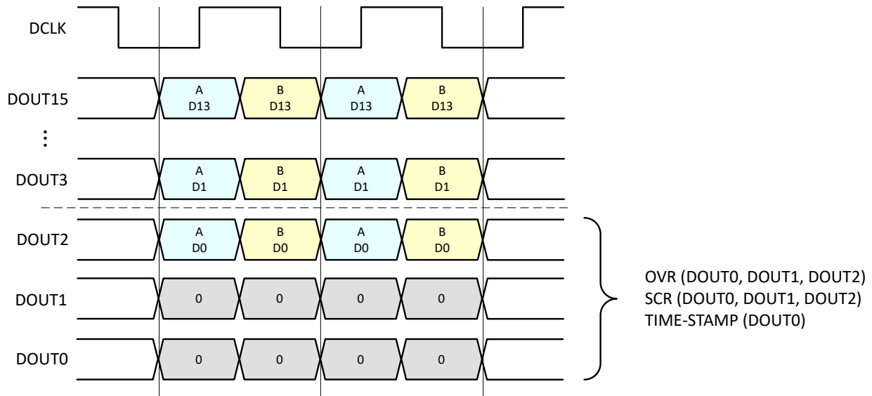
Figure 8-55. Output data format in DDR LVDS mode
