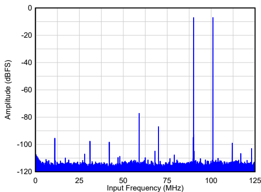
A_{IN} = -7\text{dBFS}/\text{tone} , IMD3 = 91dBc
