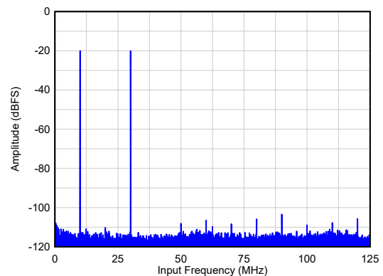
A_{IN} = -20\text{dBFS}/\text{tone} , IMD3 = 87dBc
