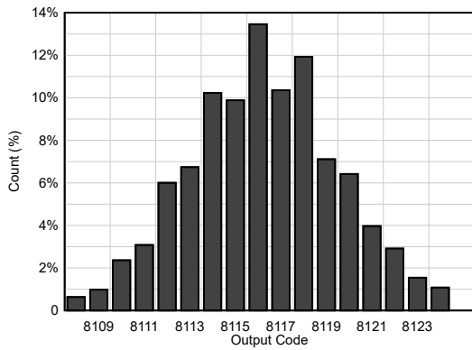
Figure 6-25. DC Offset Histogram
