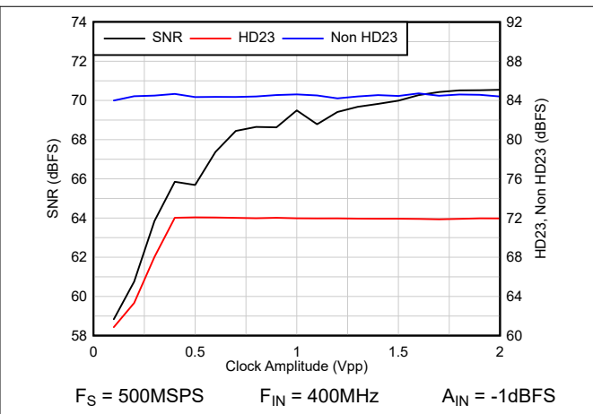
Figure 8-12. AC vs Clock Amplitude
