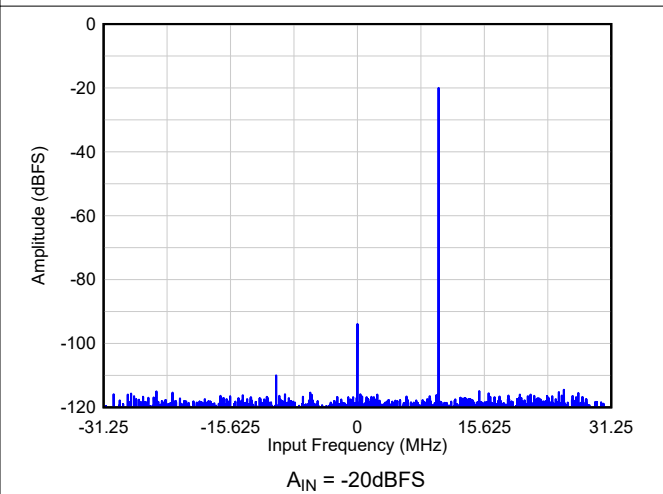
Figure 9-7. FFT4: Decimation by 8
