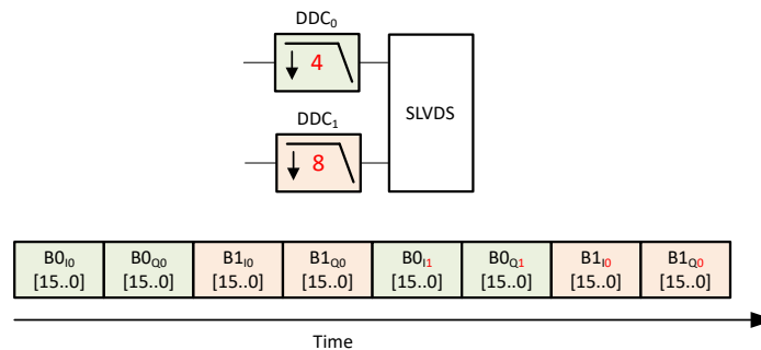
Figure 8-21. Unequal Decimation Factors
