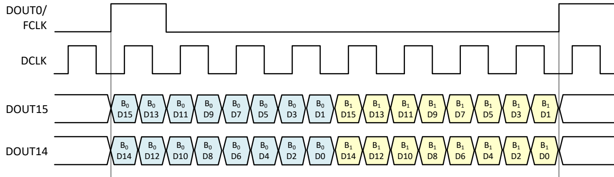
Figure 8-56. SLVDS frame assembly for example 1
