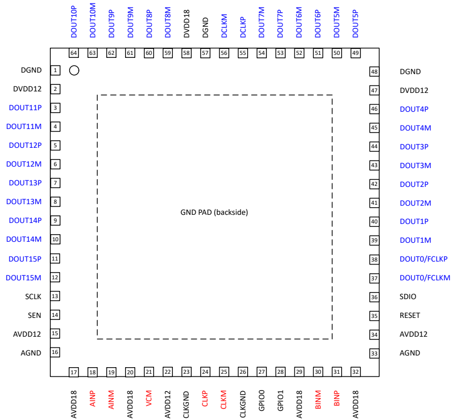
Figure 5-1. RTD Package, 64 Pin VQFN (Top View)
