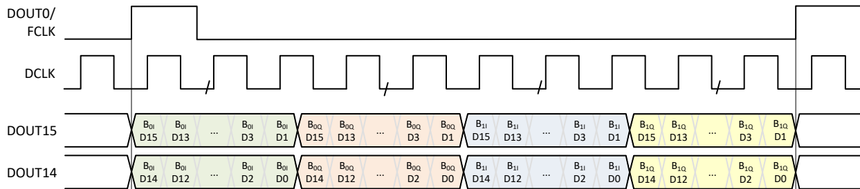
Figure 8-58. SLVDS frame assembly for example 3
