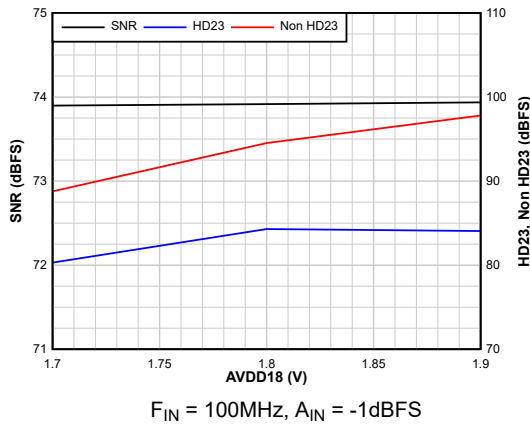
Figure 6-19. AC Performance vs AVDD18
