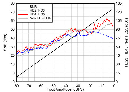
Figure 6-14. AC Performance vs A_{IN}
