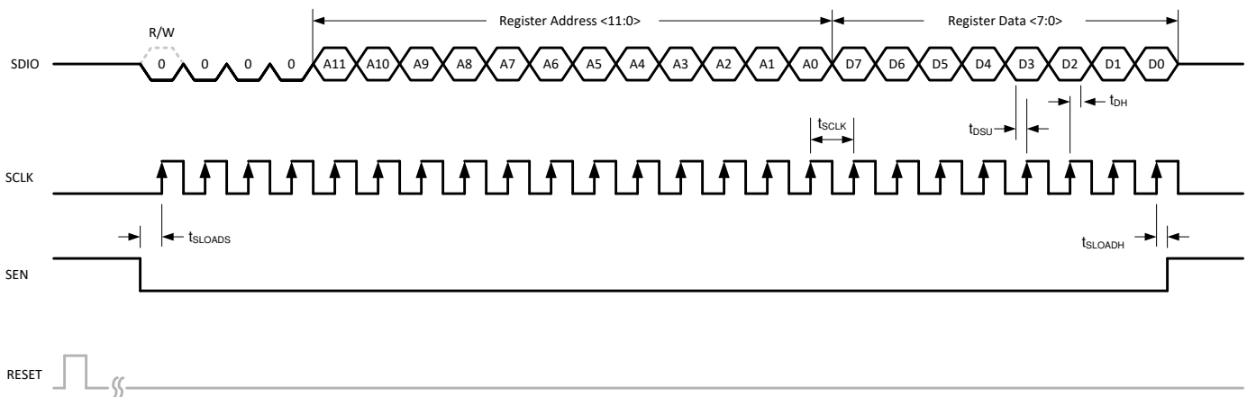
Figure 8-75. Serial Register Write Timing Diagram
