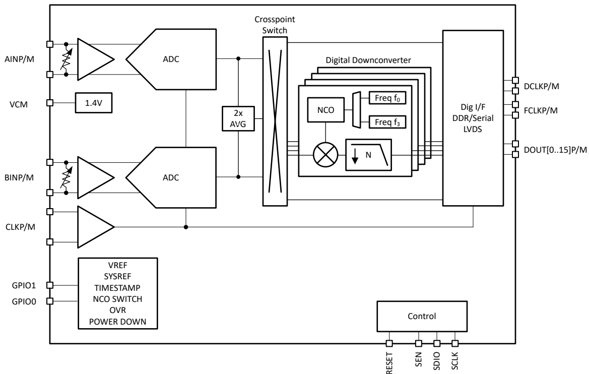
Figure 8-1. Block Diagram
