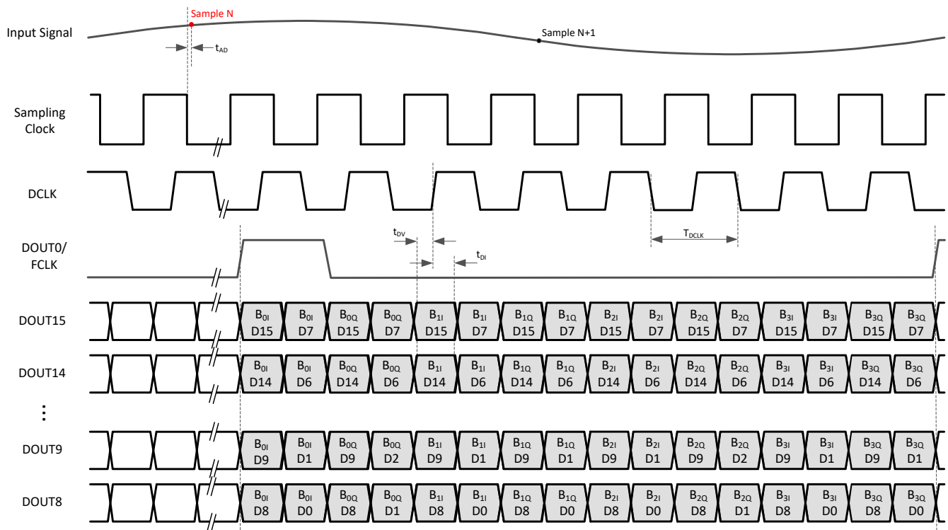
Figure 7-2. Timing Diagram - Serial LVDS (example: dual band, 16-bit, complex decimation by 8)
