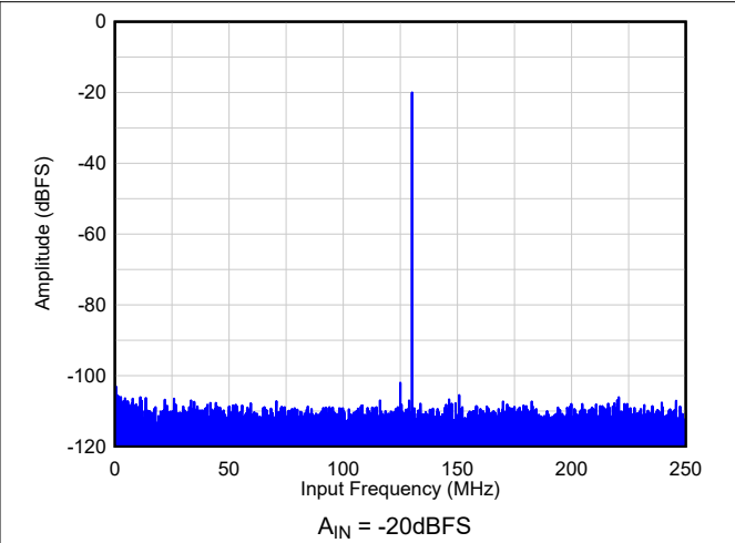
Figure 9-5. FFT2: DDC bypass
