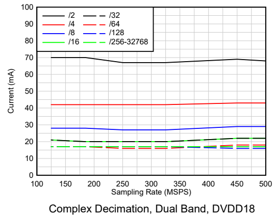
Figure 6-58. Current vs Sampling Rate
