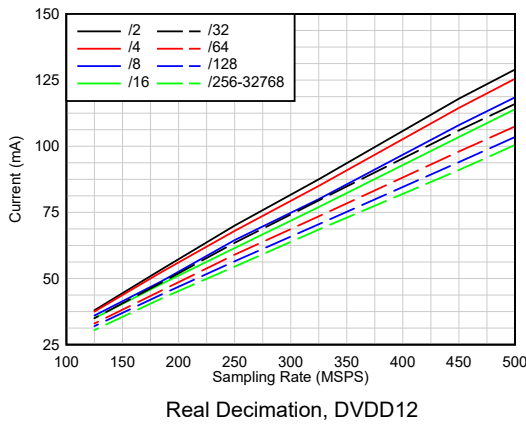
Figure 6-57. Current vs Sampling Rate
