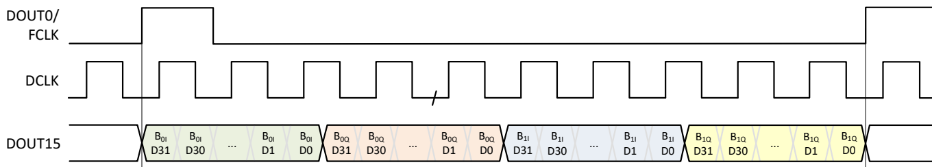
Figure 8-60. SLVDS frame assembly for example 5
