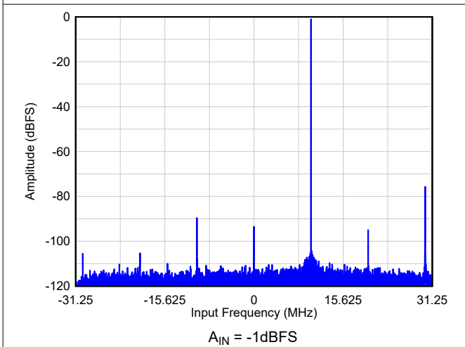
Figure 9-6. FFT3: Decimation by 8
