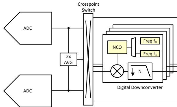
Figure 8-53. NCO Block Diagram
