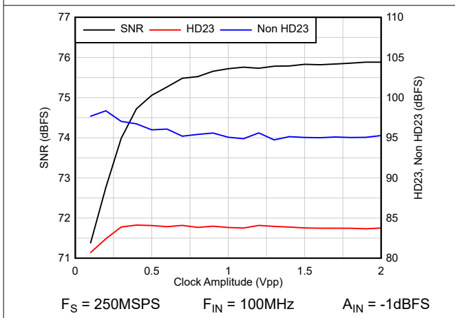
Figure 8-13. AC vs Clock Amplitude
