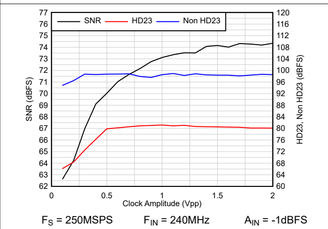
Figure 8-14. AC vs Clock Amplitude
