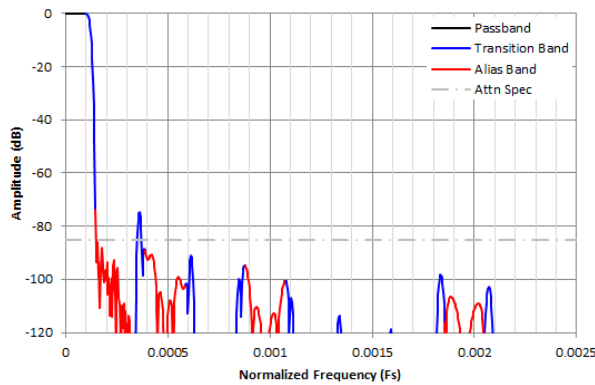
Figure 8-45. Complex Decimation by 4096 Filter Response
