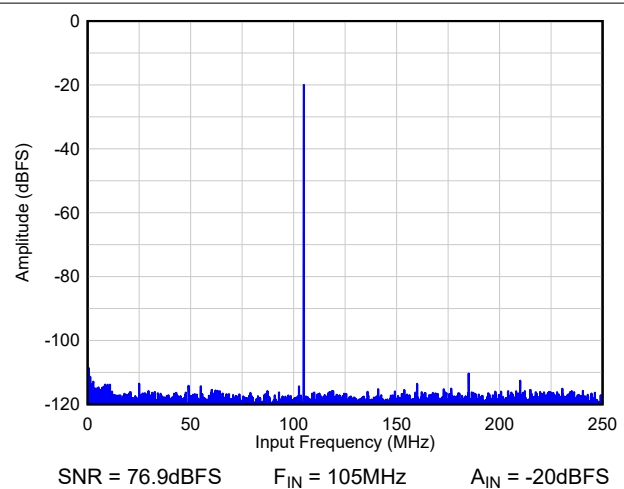
Figure 8-74. FFT - 2x AVG
