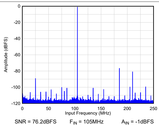
Figure 8-72. FFT - 2x AVG
