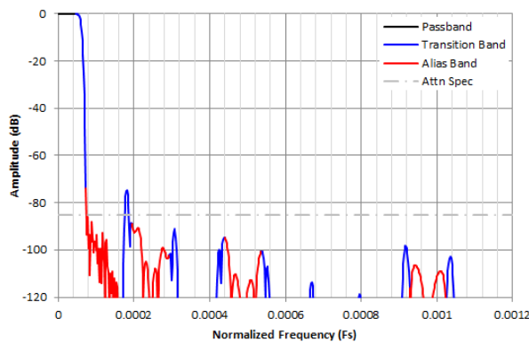
Figure 8-47. Complex Decimation by 8192 Filter Response
