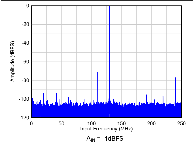
Figure 9-4. FFT1: DDC bypass
