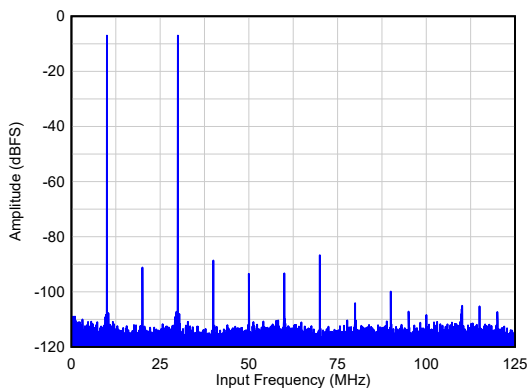
A_{IN} = -7\text{dBFS}/\text{tone} , IMD3 = 83dBc
