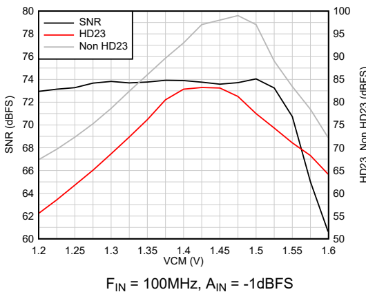
Figure 6-21. AC Performance vs VCM
