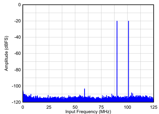
A_{IN} = -20\text{dBFS}/\text{tone} , IMD3 = 99dBc
