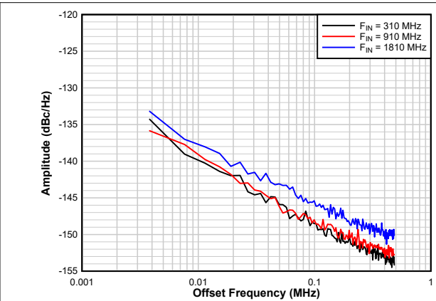
Figure 8-10. Amplitude Noise Examples
