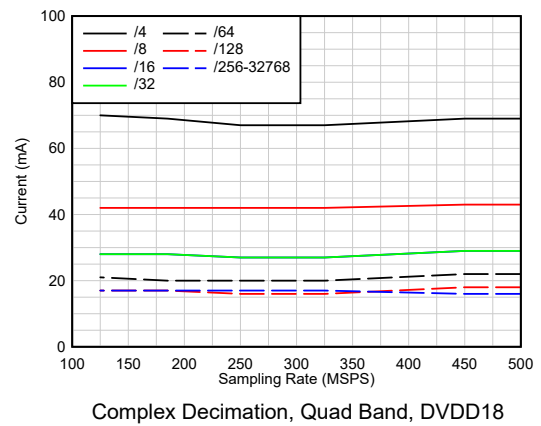
Figure 6-60. Current vs Sampling Rate
