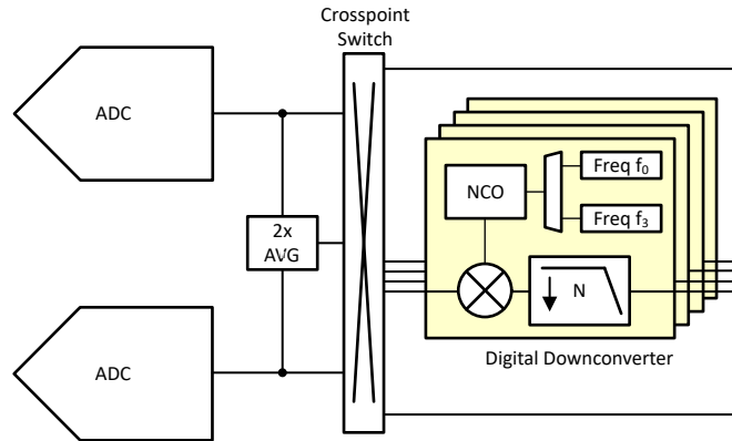
Internal digital down converter
