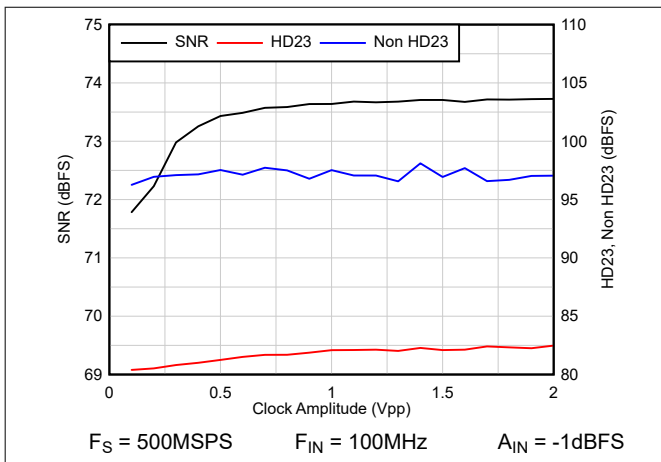
Figure 8-11. AC vs Clock Amplitude
