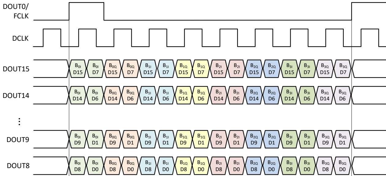
Figure 8-59. SLVDS frame assembly for example 4
