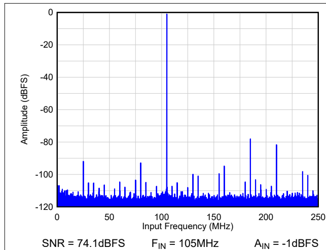
Figure 8-71. FFT - no AVG
