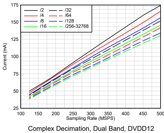
Figure 6-59. Current vs Sampling Rate
