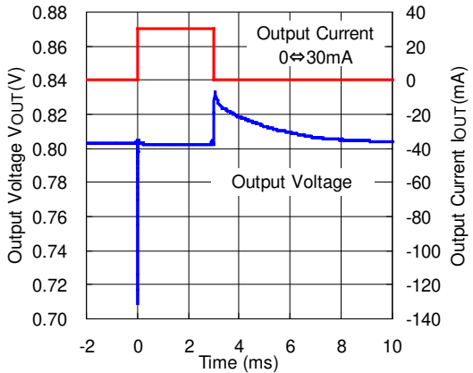
RP202x28xx (Auto ECO Low Power Mode ↔ FAST Mode) V_{IN}=3.8V
