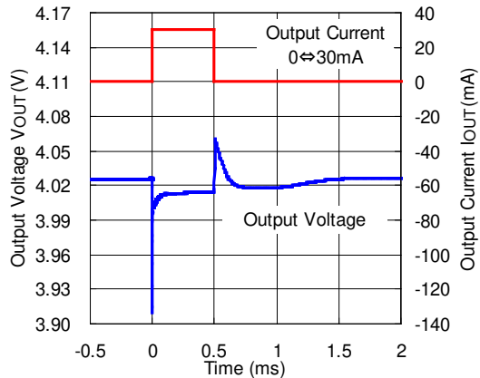
RP202x40xx (Auto ECO Low Power Mode ↔ FAST Mode) V_{IN}=5.0V
