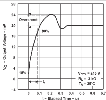
Figure 5-56. Output Voltage vs Elapsed Time
