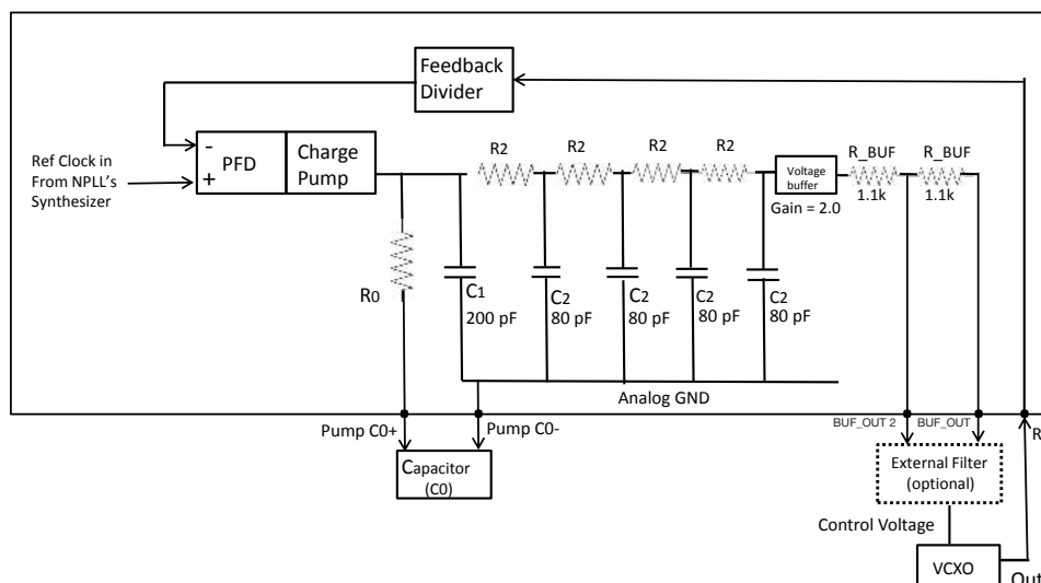
APLL Circuit Diagram
