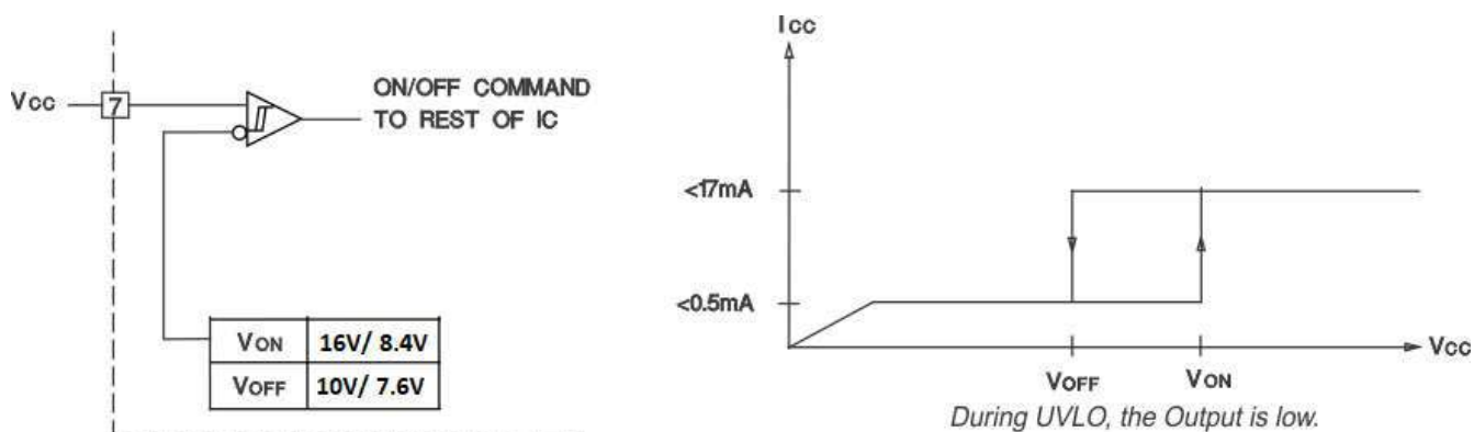
Figure 7-3. Undervoltage Lockout
