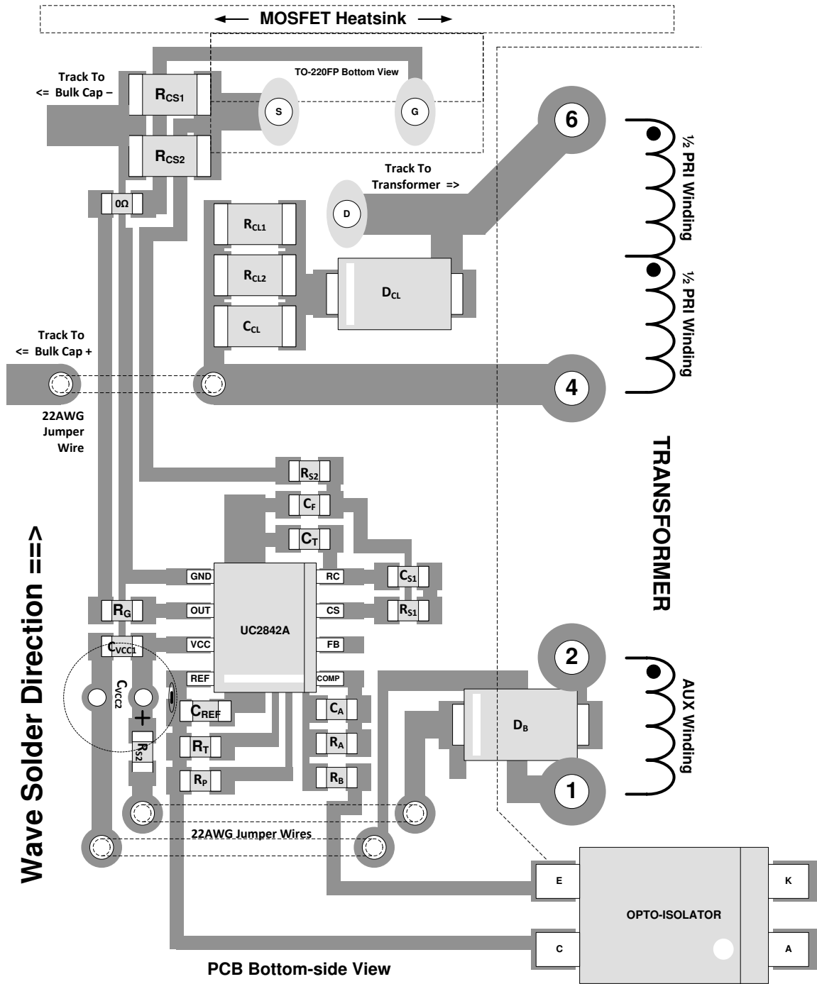
Figure 8-6. Layout Diagram
