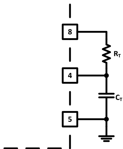
Figure 7-4. Oscillator Section
