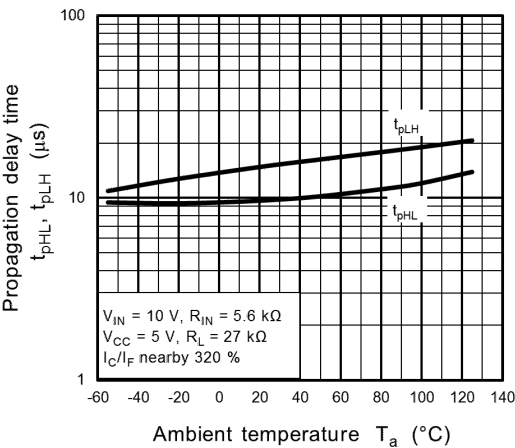
Fig. 11.17 Propagation delay Time - T_a
