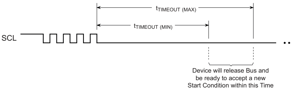
Figure 10-2. SMBus Timeout
