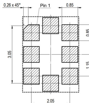
Figure 4. Recommended land pattern. All dimensions in millimeters.
