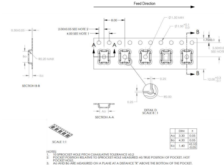
Figure 7. Technical drawing of tape and reel packaging. All dimensions in millimeters.
