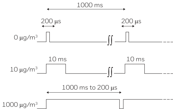
Figure 5. PWM output timing diagram
