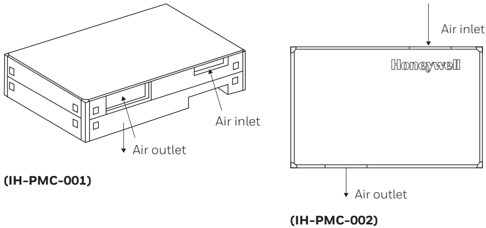
Figure 8. PM 2.5 Airflow
