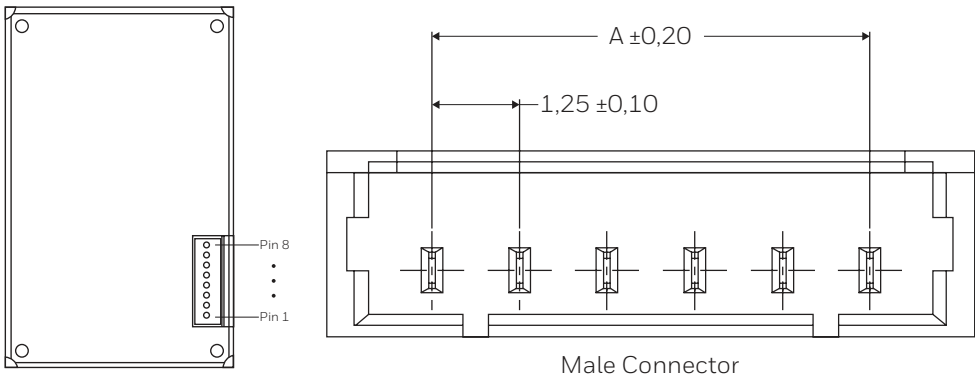
Figure 3. PM 2.5 pinout and connector details
