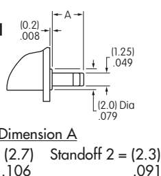
Standoff Detail
