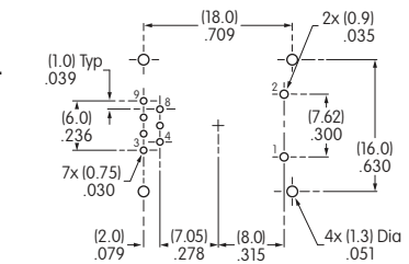
Footprint
