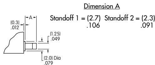
Standoff Detail
