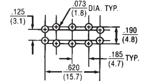
2 Pole P.C. Mounting
