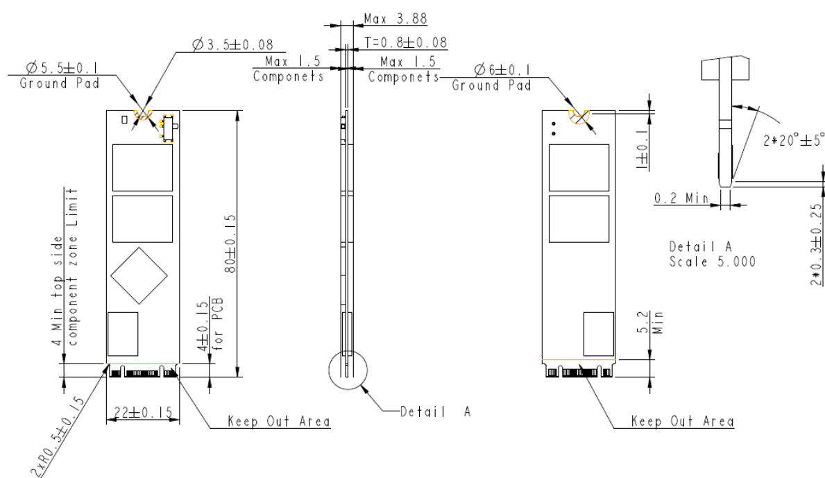
Figure 9-1 Physical Dimensions
