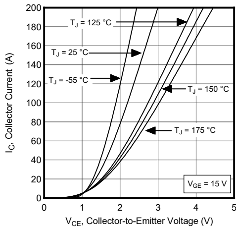
Figure 1-1. Output Characteristics
