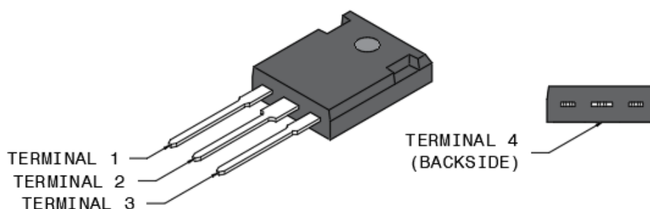
Figure 2-2. Terminal Pinout
