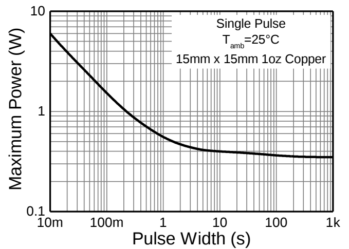
Figure 4. Pulse Power Dissipation
