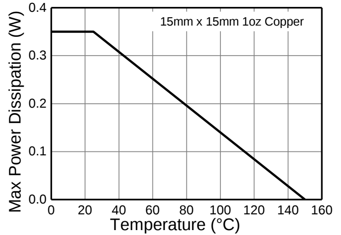
Figure 2. Derating Curve
