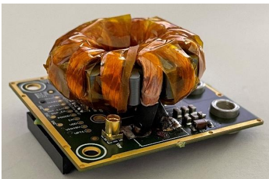
Figure 14: EPCS401 with air-core 220nH inductor.
