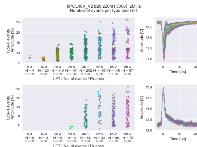
Figure 24. Single Event Transients
