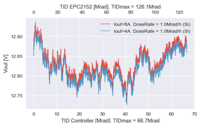
Figure 23. EPCSC401 Vout vs TID. -30°C temperature.
