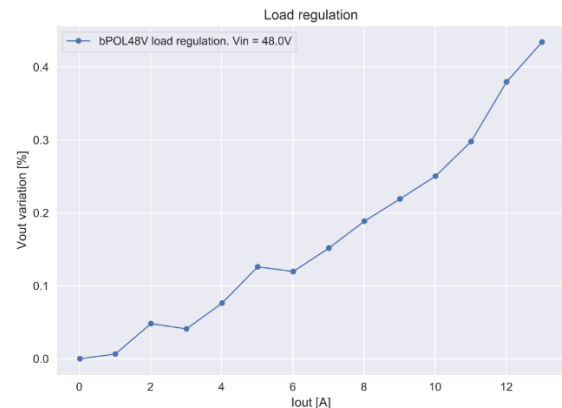
Figure 20: EPCSC401 Load regulation characteristic
