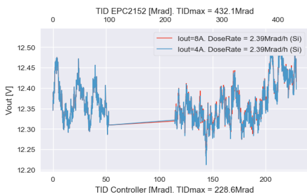
Figure 22. EPCSC401 Vout vs TID. Ambient temperature. Note: Acquisition failed between 52Mrad and 114Mrad
