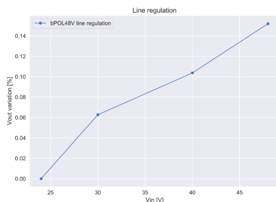
Figure 21: EPCSC401 Line regulation characteristic
