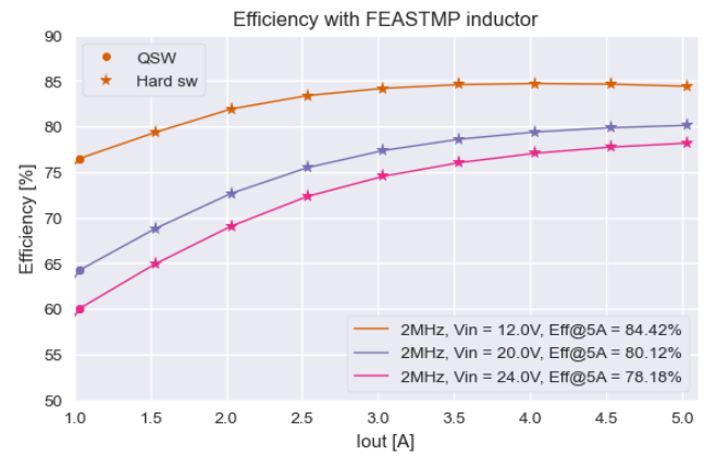
Figure 19: Efficiency of EPCSC401 with 460nH small air-core inductor and V_{out}=2.5V .
