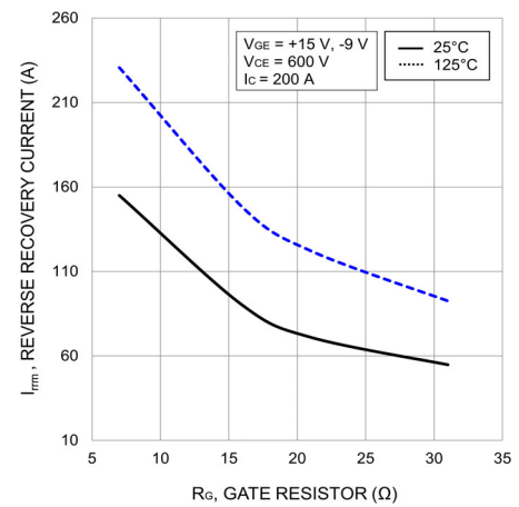
Figure 53. Typical Reverse Recovery Peak Current vs. R_G
