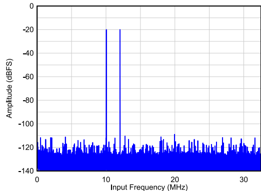
Figure 5-9. Two Tone FFT at F_{IN} = 10/12\text{MHz}
