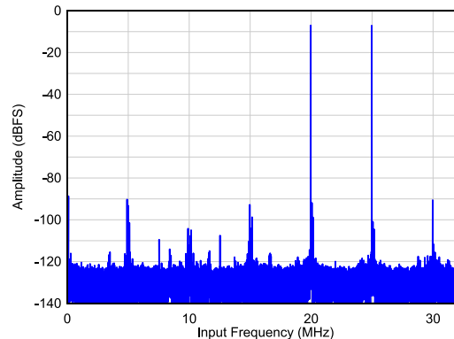
Figure 5-10. Two Tone FFT at F_{IN} = 40/45\text{MHz}
