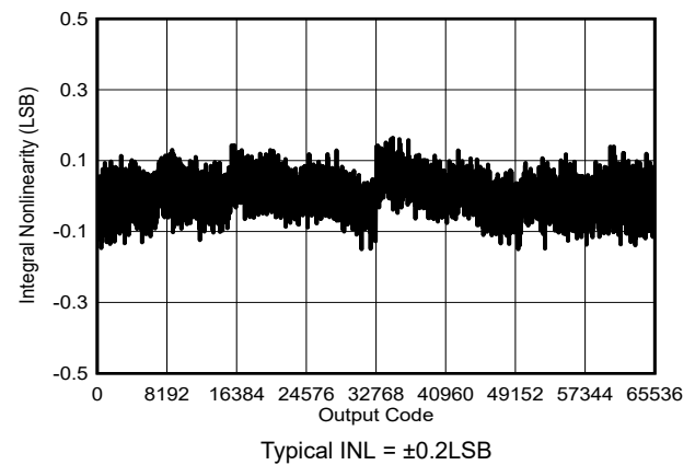
Figure 9-3. Typical INL
