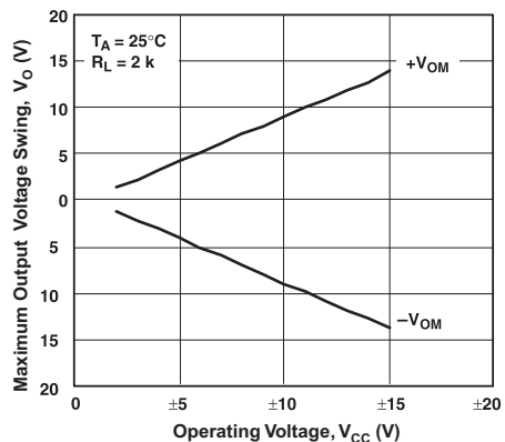
Figure 5-9. Maximum Output Voltage Swing vs Operating Voltage
