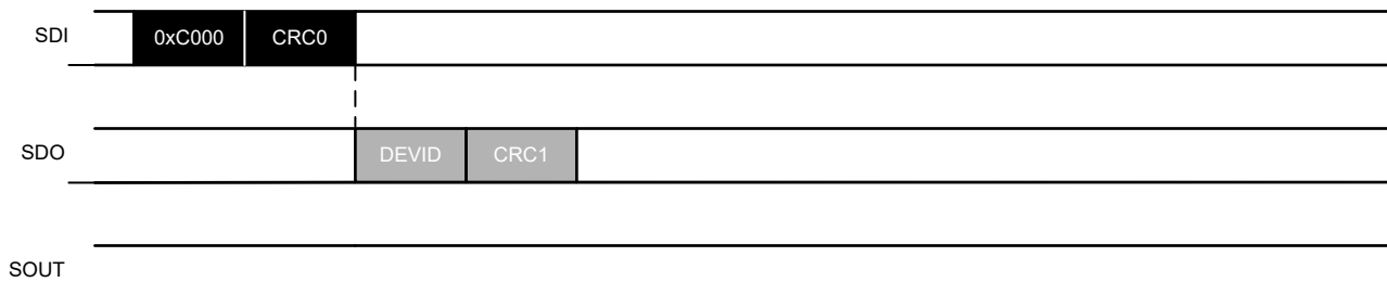
Figure 7-19. Example of REG_RD_CRC command
