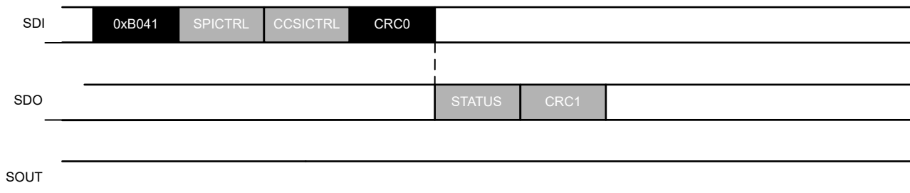
Figure 7-18. Example of REG_WR command
